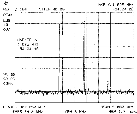
Figure 3-25. Measuring the Distortion Product
