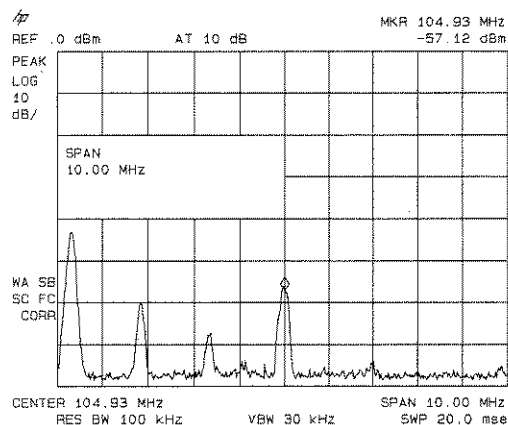
Figure 3-16. Low-Level Signal
