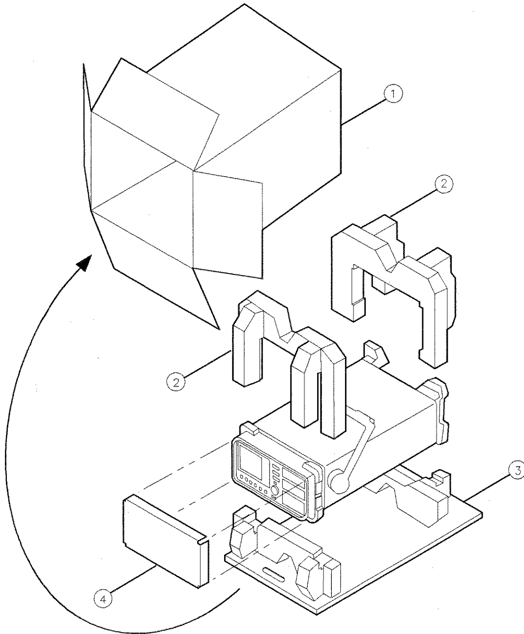
Figure 8-1. HP 8590 Series Packaging
