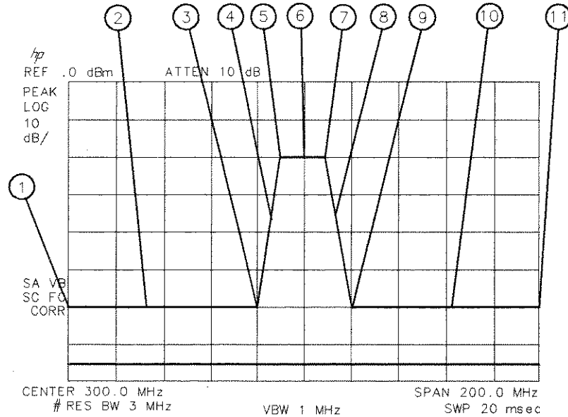
Figure 5-6. Limit-Line Segments
