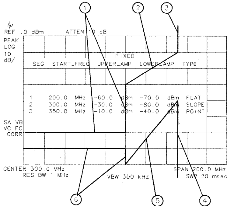
Figure 5-7. Segment Types
