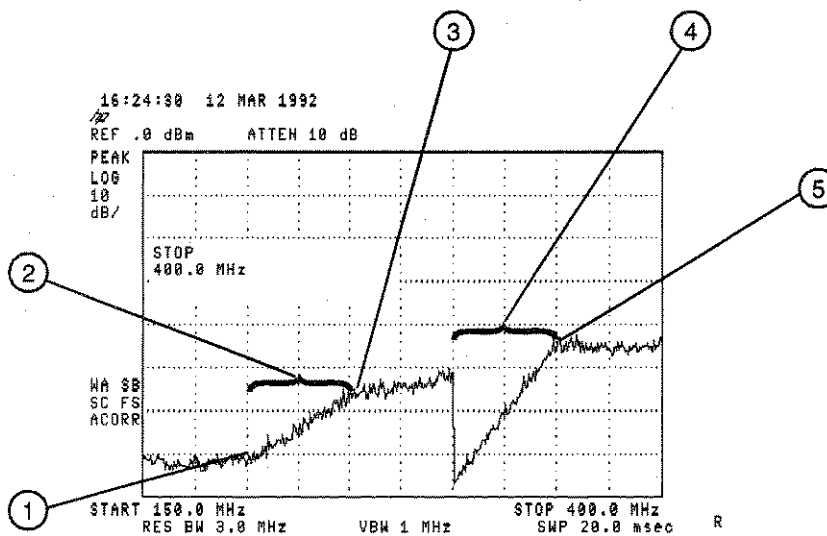
Figure 5-13. Amplitude-Correction Points
