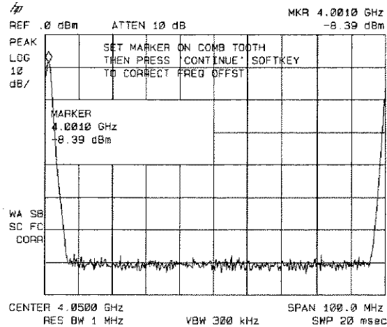
Figure 3-31. Using the Correct to Comb Function
