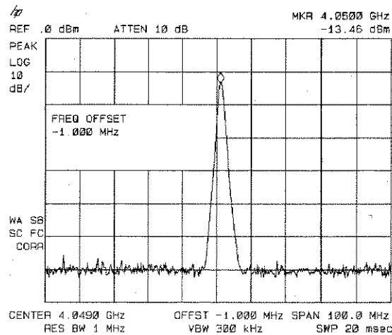
Figure 3-32. Frequency Readout with a Frequency Offset
