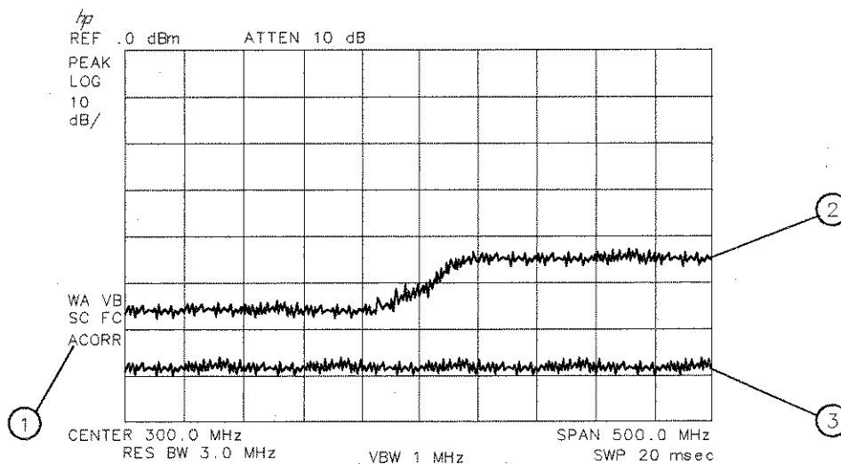
Figure 5-11. Amplitude-Correction Display
