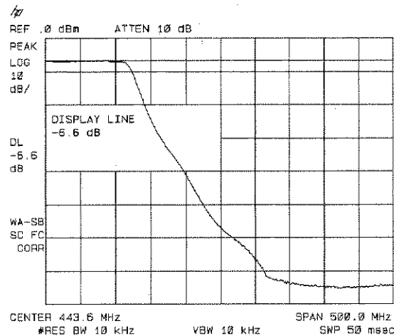
Figure 4-9. Normalized Trace
