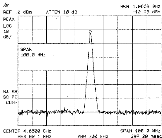
Figure 3-30. Measuring an Input Signal
