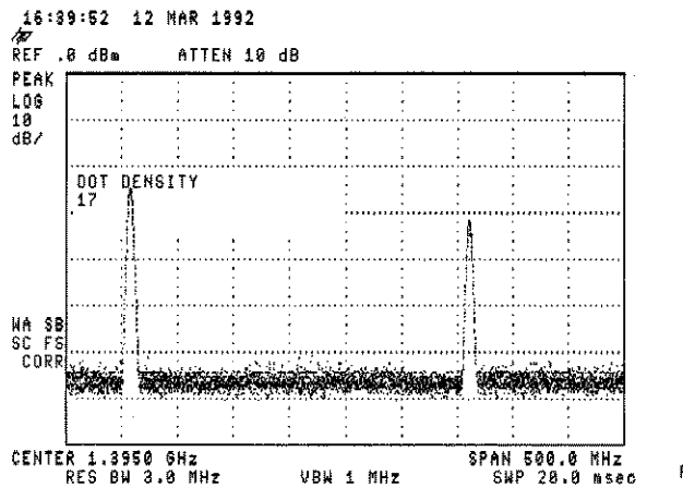
Figure 5-9. Analog+ Display Mode
