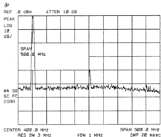
Figure 3-21. Harmonic Distortion
