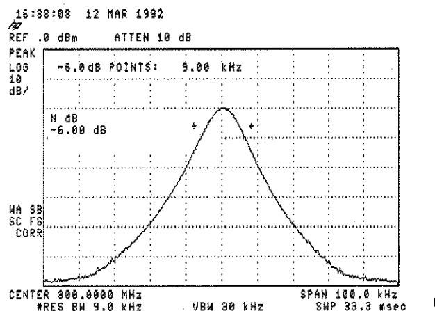
Figure 4-34. N dB Bandwidth Measurement
