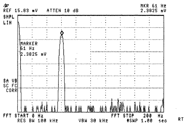
Figure 4-1. FFT Annotation
